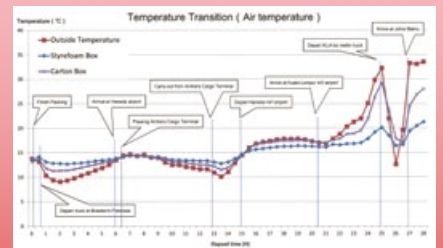
Change in Temperatures during Shipment from Niigata to Malaysia on April 3, 2017
